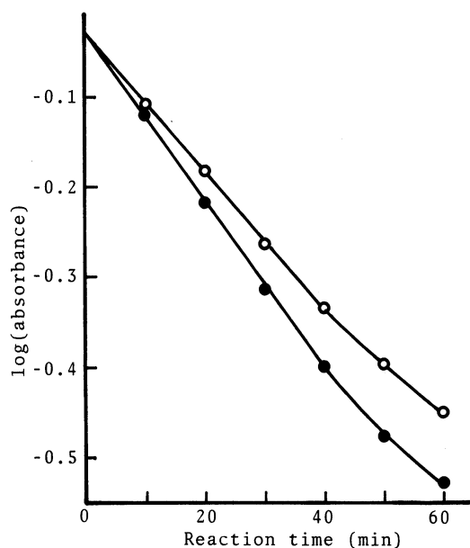
Fig. 1. First-order plots for the iodine-cerium(IV) reaction. (○) Blank ; (●) 2 µg manganese per 16.5 ml. Conditions : 7.2 \times 10^{-4} M iodide ; 2.4 \times 10^{-2} M cerium(IV) ; 1.6 M nitric acid ; 1.2 \times 10^{-2} M dichromate ; 20°C.
