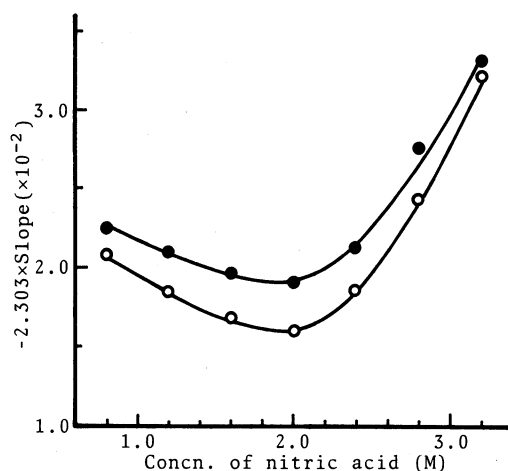
Fig. 2. Effect of nitric acid concentration.
