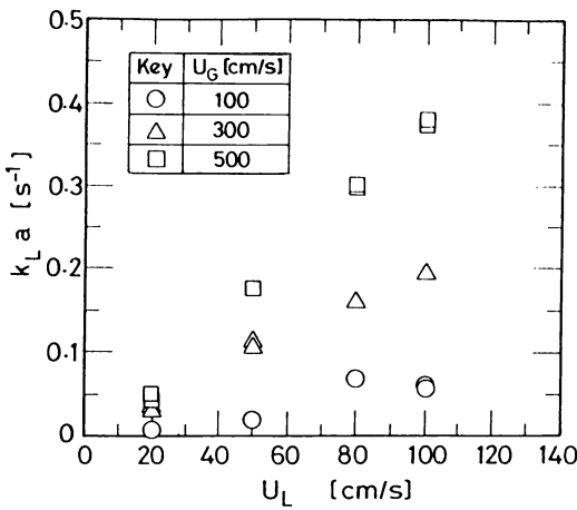
Fig. 5 Effect of gas velocity on volumetric coefficient in gas-liquid two-phase flow
