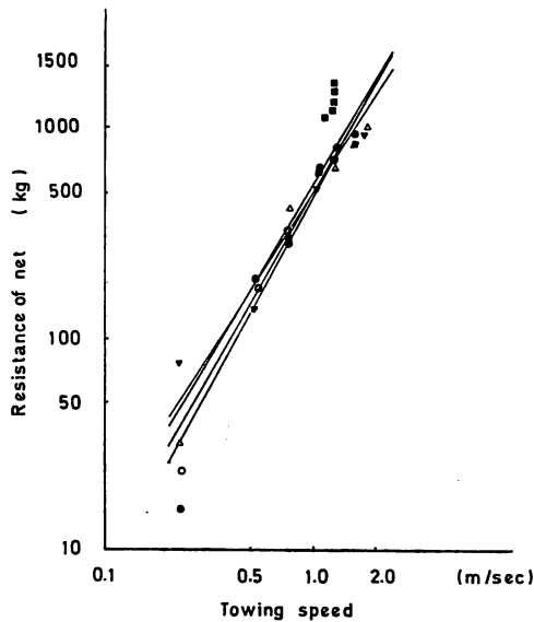
Fig. 10. Relationship between the towing speed and the net resistance on six-seam net. Symbols in figure show the distance between both wing tips; (o): 4.6 m, (v): 6.1 m, ( \Delta ): 7.6 m, ( \bullet ): 9.1 m, ( \blacksquare ): Field data.
