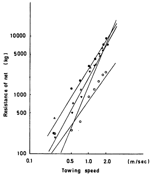
Fig. 9. Relationship between the towing speed and the net resistance on four-seam-net. Symbols in figure show the distance between both wing tips; (o): 14.3 m, (v): 19.1 m, ( \Delta ): 23.8 m, ( \bullet ): 28.6 m.
