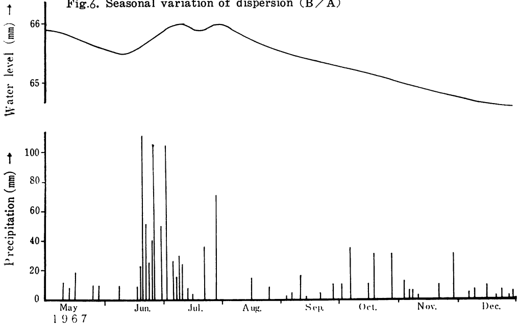
Fig. 7. Seasonal variation of priation of precipitation and water level.
