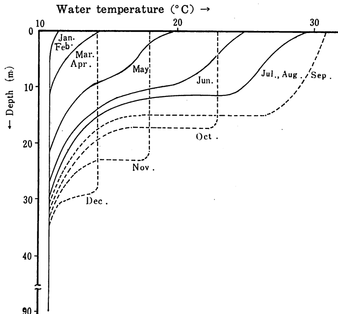
Fig. 4. Seasonal variation of distribution of water temperature. (Lake—Ikeda) 1967
