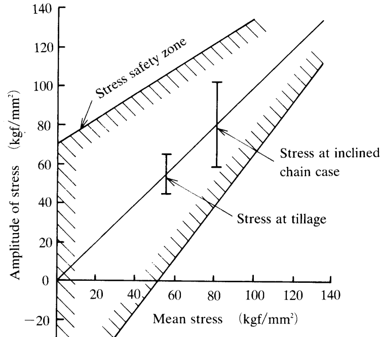
Fig. 9. Measured stress and fatigue limit diagram of SK5P.
