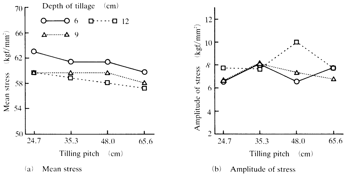
Fig. 5. Influence of tilling pitch.
