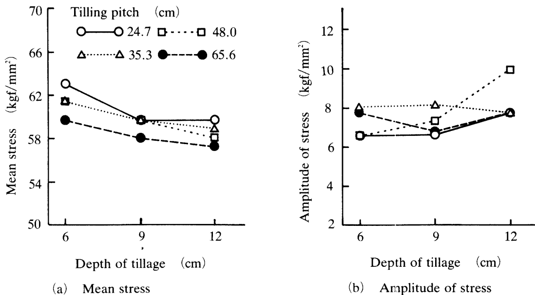
Fig. 4. Influence of depth of tillage.
