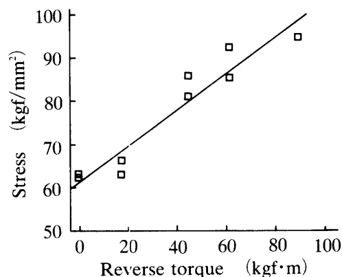
Fig. 8. Stress at reverse torque.
