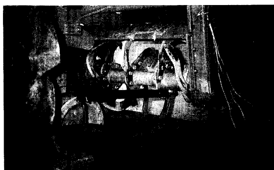
Fig. 7. Measurement of stress at reverse torque.
