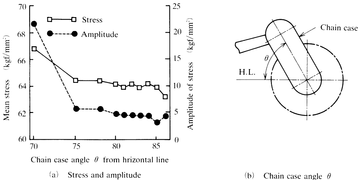
Fig. 6. Influence of the inclination of the chain case.
