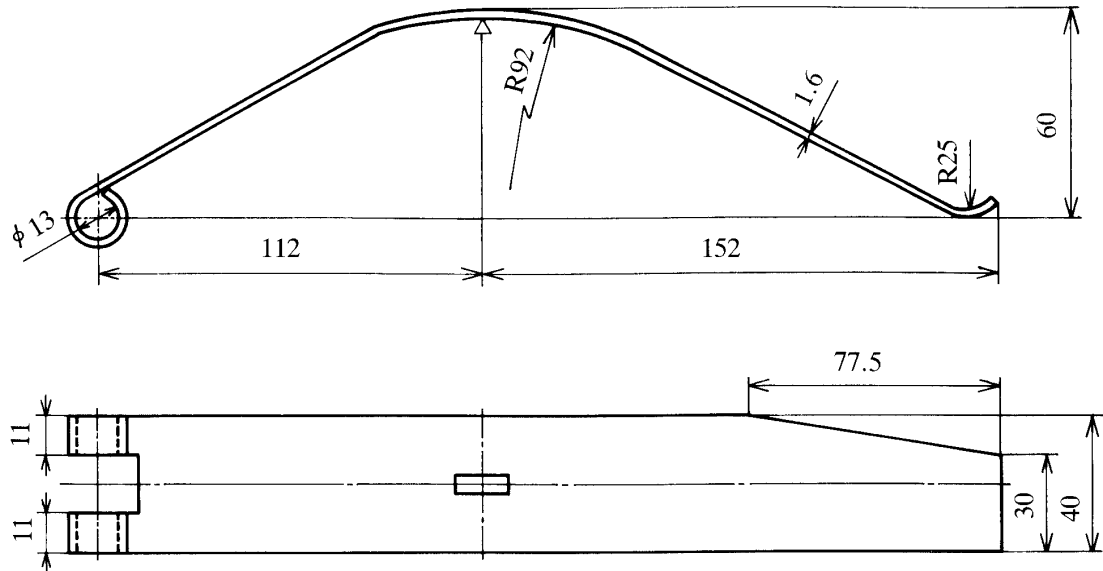
Fig. 1. Sketched shape of the tested tightener and location of attached gauge.
