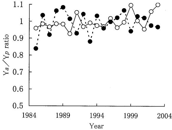
Fig. 6 Changes in the ratio of actual yield ( Y_a ) to meteorologically potential yield ( Y_p ) ( Y_a/Y_p ) on early and normal season cultures from 1985 to 2003 at Kagoshima City. *The values are shown in the ratio to average from 1985 to 2003. Symbols are the same as those shown in Fig. 2.
