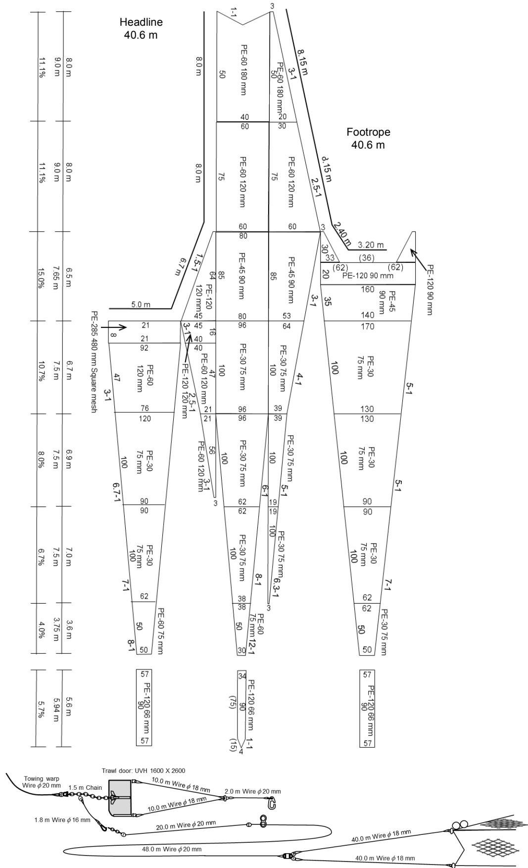
Fig. 2 Diagram of bottom trawl net used onboard the T/V Kagoshima-maru during academic year 2014 (April, 2014 - March, 2015).
