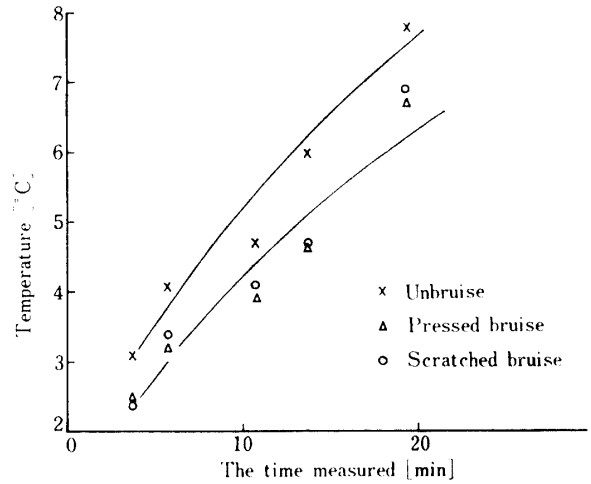
Fig. 7. Relationship between temperature changes at the bruised Japanese pear and the time measured.
