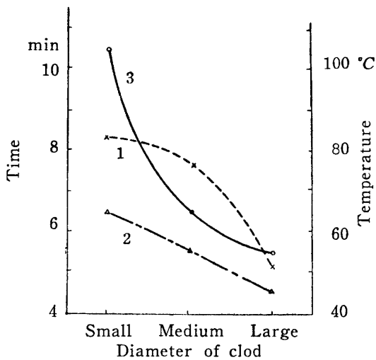
Fig. 10. Effect of diameter of soil clod on the time and the temperature. Curve 1: Time needed to make 55°C soil temperature at 3cm depth. Curve 2: Soil temperature at 3cm depth 2 seconds after stopped burning. Curve 3: Soil surface temperature at the same time as Curve 2.
