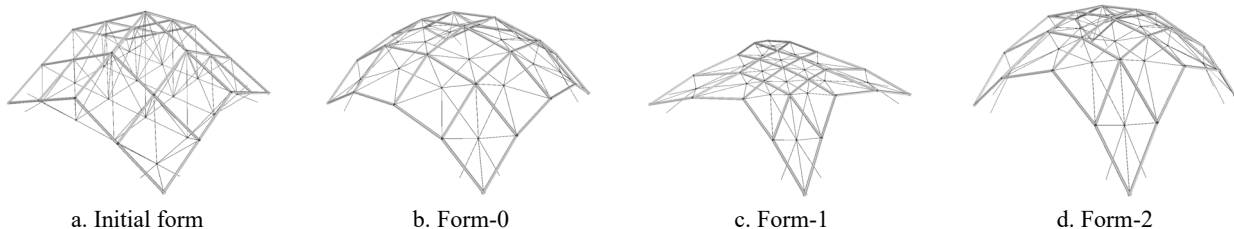
Figure.1 Structural form of hybrid structure constituting self-equilibrated state with cable and strut
