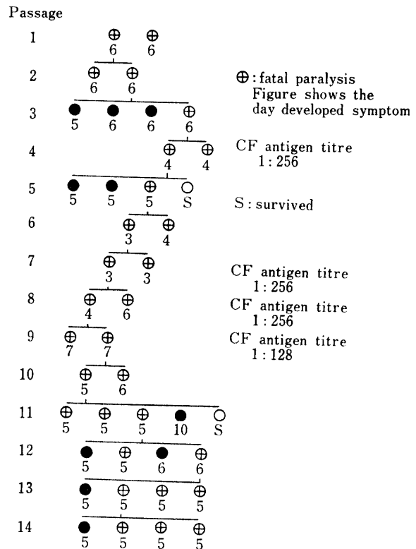
Fig. 3. Nodamura virus passage in young gpc mice. Filled circle shows mouse which died without symptom.
