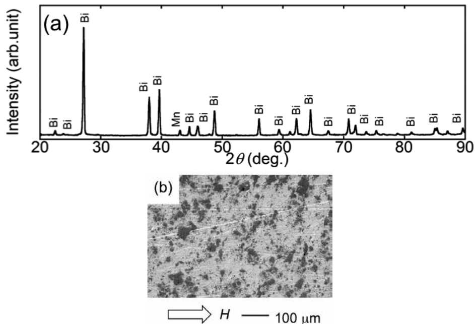
Fig. 3. (a) The powder XRD patterns of the sample at 513 K for 24 h at a magnetic field of \mu_0 H = 15 T (b) The microstructure at 513 K for 24 h at a magnetic field of \mu_0 H = 15 T.
