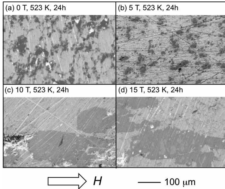
Fig. 2. The microstructure at 523 K for 24 h at magnetic fields of \mu_0 H = 0 T (a), 5 T (b), 10 T (c), and 15 T (d).
