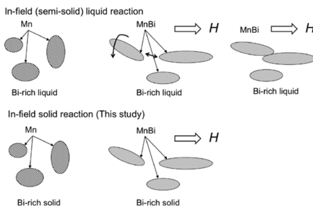
Fig. 4. The schematic model in field reaction for this experimentation.
