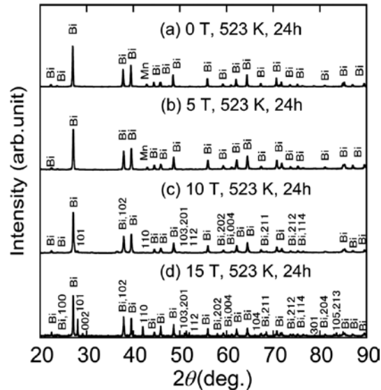
Fig. 1. The powder XRD patterns of the samples at 523 K for 24 h at magnetic fields of \mu_0 H = 0 T (a), 5 T (b), 10 T (c), and 15 T (d).
