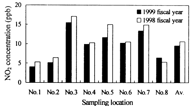
Fig. 13 Average concentration of \text{NO}_2 for 8 locations in Kagoshima City
