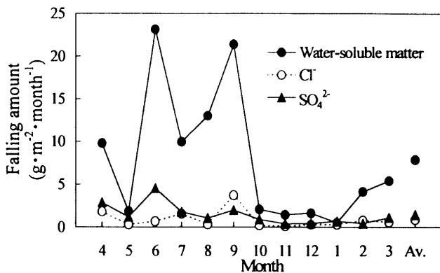
Fig. 11 Average of falling water-soluble matter, \text{SO}_4^{2-} , and \text{Cl}^- for 8 locations in Kagoshima City
