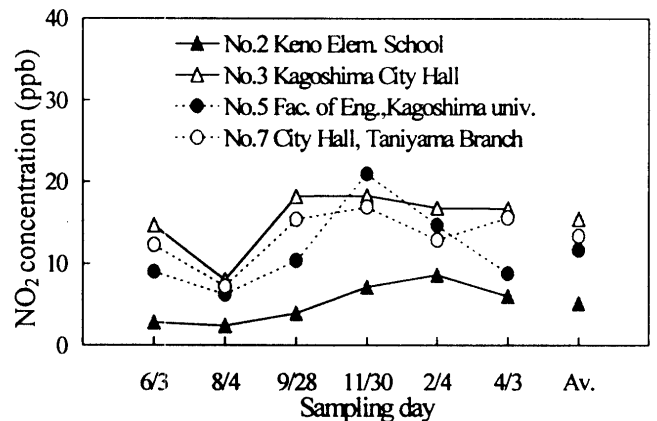
Fig. 14 \text{NO}_2 concentrations at 4 locations
