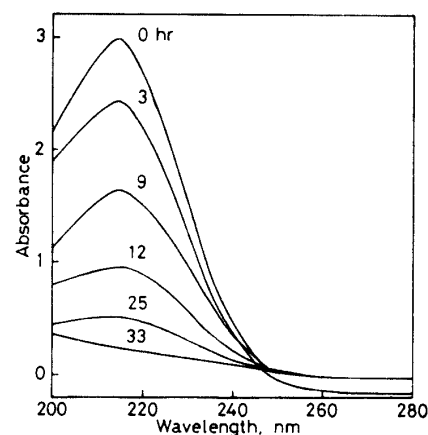
Fig. 5. Changes of UV spectrum in catalytic reduction of cycasin in neutral medium.
