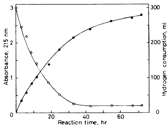
Fig. 4. Development of catalytic reduction of cycasin in neutral medium. Open circle: absorption at 215 nm. Closed circle: hydrogen-consumption.
