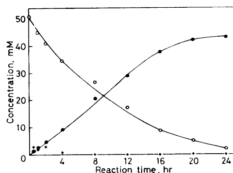
Fig. 2. Development of reduction of cycasin with \text{NaBH}_4 , analyzed by GC. Open circle: cycasin. Closed circle: sorbitol. Cross: glucose.
