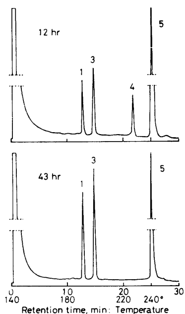
Fig. 6. Gas chromatogram of the products in catalytic reduction of cycasin. Samples: at 12 and 43 hr-reaction. Chromatography: same as in Fig. 1. Peaks: 1, \alpha -glucose 3, \beta -glucose 4, cycasin 5, androsterone (inner standard).
