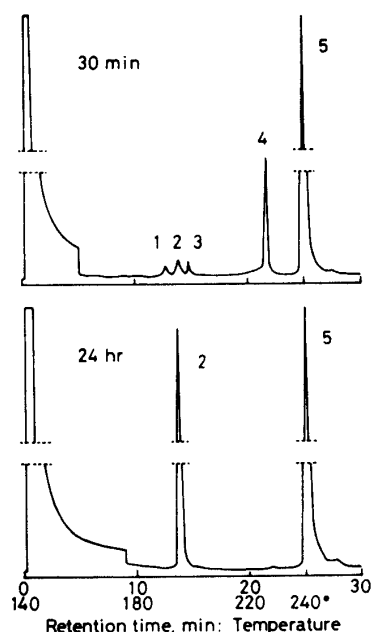
Fig. 1. Gas chromatogram of the products from cycasin reduced with \text{NaBH}_4 . Samples: at 30 min- and 24 hr-reaction. Column: SE-52, 3 mm \times 1.5 m. Program: 140° – 240°, 4°/min. Carrier: \text{N}_2 . Peaks: 1, \alpha -glucose 2, sorbitol 3, \beta -glucose 4, cycasin 5, androsterone (inner standard).
