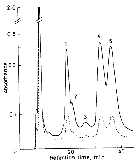
Fig. 3. Amines produced in reduction of cycasin with \text{NaBH}_4 , analyzed by amino acid analyzer. Solid line: 570 nm. Broken line: 440 nm. Peaks: 1, 2, 3, unknowns 4, ammonia 5, methylamine.
