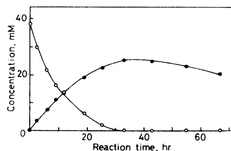
Fig. 7. Development of catalytic reduction of cycasin in neutral medium. Open circle: cycasin. Closed circle: glucose.
