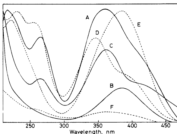
Fig. 8. UV and visible spectra of DNP-amine A – F, derived from the products in catalytic reduction of cycasin in acidic medium.
