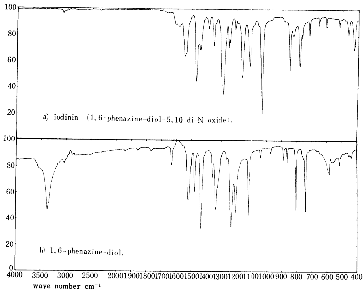
Fig. 4. Infrared spectra : a) iodinin from Br. stationis var. iodinofaciens (Found : C, 58.89; H, 3.47; N, 11.19. C_{12}H_8O_4N_2 requires C, 59.02; H, 3.30; N, 11.47%); b) 1,6-phenazine-diol, to which iodinin was not reduced only chemically, but also biologically under anaerobic conditions (Found : C, 66.58, 66.38; H, 3.81, 4.05; N, 12.83. C_{12}H_8O_2N_2 requires C, 67.97; H, 3.80; N, 13.28 %).
