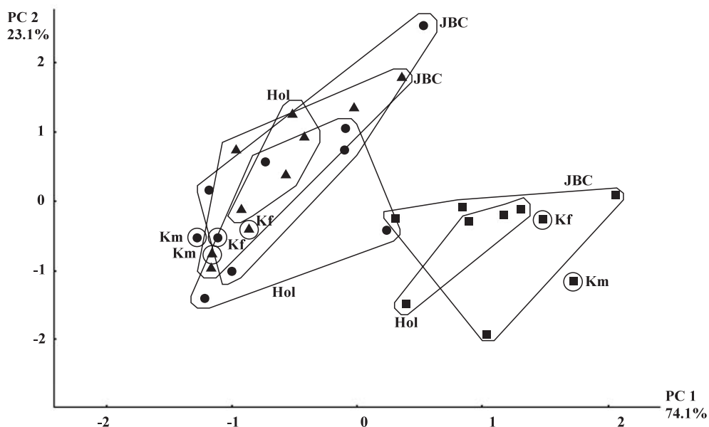
Fig. 2. Principal component chart for the first and second transformed variable of myofiber types of M. longissimus thoracis . ●: type I myofiber, ▲: type II myofiber, ■: intermediate type of myofiber. Kf: female Kuchinoshima feral cattle, Km: male Kuchinoshima feral cattle, JBC: Japanese black cattle, Hol: Holstein steer.
