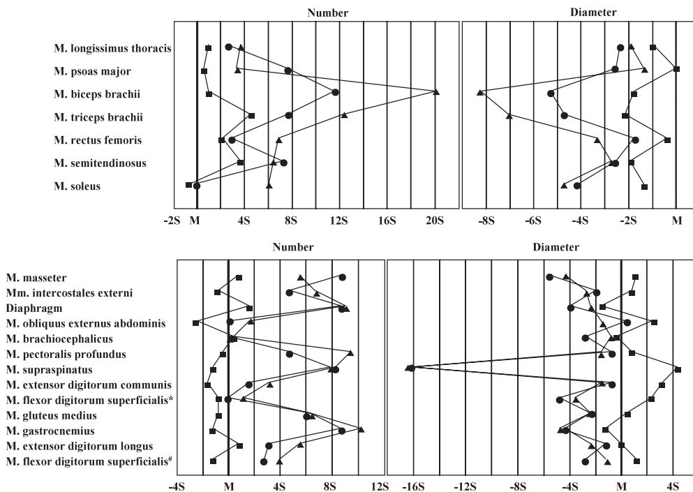
Fig. 3. Deviation graphs on the number and diameter of muscle fibers. M: mean of Japanese black cattle, S: standard deviation. ●: female Kuchinoshima feral cattle, ▲: male Kuchinoshima feral cattle, ■: Holstein steer. *: thoracic limb, #: pelvic limb.
