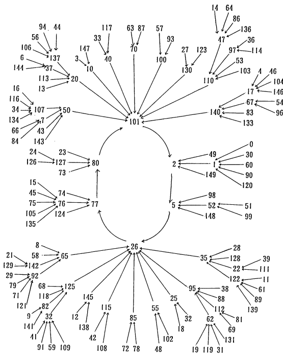
The iteration graph of the case when f(x) = x^2 + 1 \pmod{150} ( x \in \mathbf{Z}_{150} )
