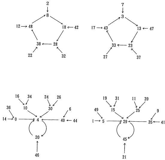
(e) The iteration graph of the case when f(x) = x^2 + 4 \pmod{50} ( x \in \mathbf{Z}_{50} )
