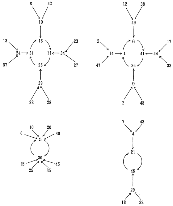
(f) The iteration graph of the case when f(x) = x^2 + 5 \pmod{50} ( x \in \mathbf{Z}_{50} )
