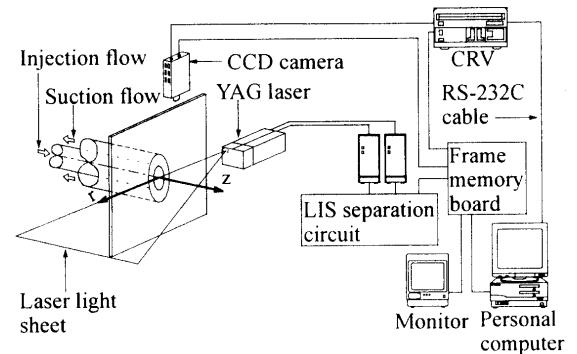
Fig.1 Schematics of visualization system and image processing system
