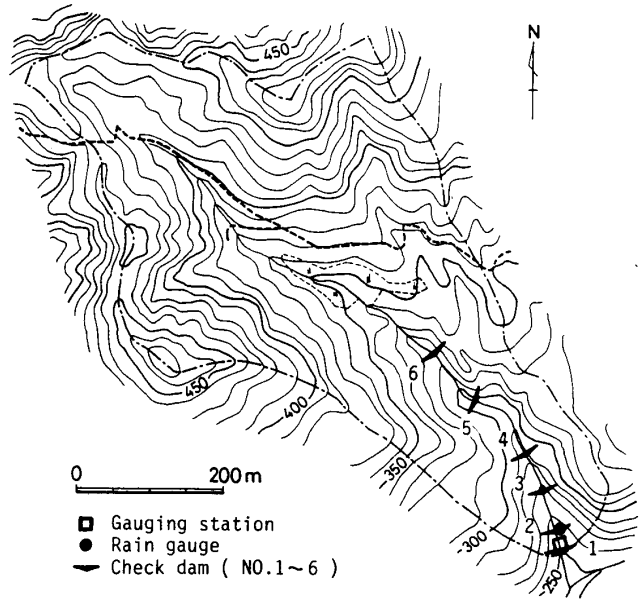
Fig. 2. Topography of experimental basin.
