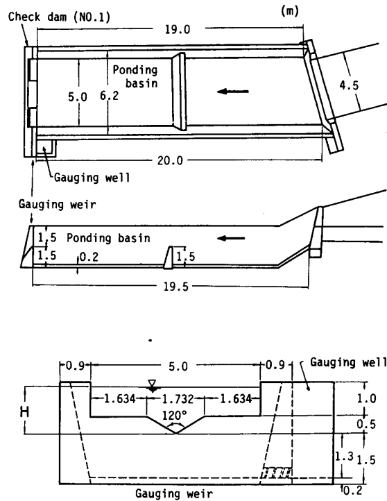
Fig. 3. Structure of gauging station.
