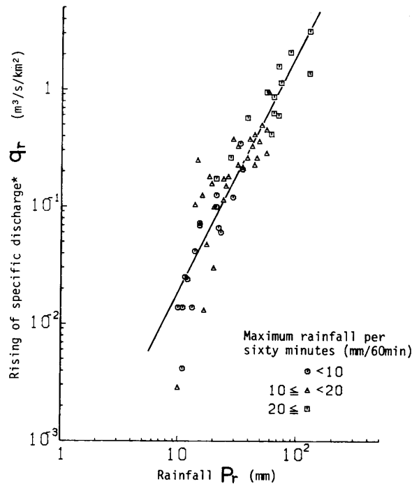
Fig. 12. Relationship between risings of specific discharge and rainfalls. * Increase in specific discharge during rising limb of hydrograph.
