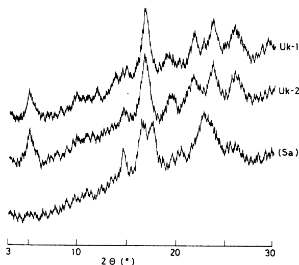
Fig. 4. X-ray diffractograms. Rigakudenki D-3F, 30kV-12mA, 1^\circ(2\theta) /min.
