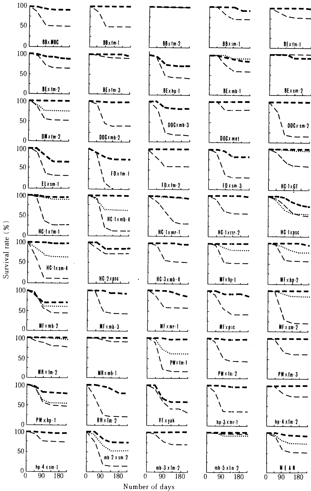
Fig. 1. The consecutive changes in the survival rate of different size seedlings. The size of seedlings : heavy broken line ; large, dotted line ; medium, fine broken line ; small. For survival rate and other items, see footnotes of Table 1.
