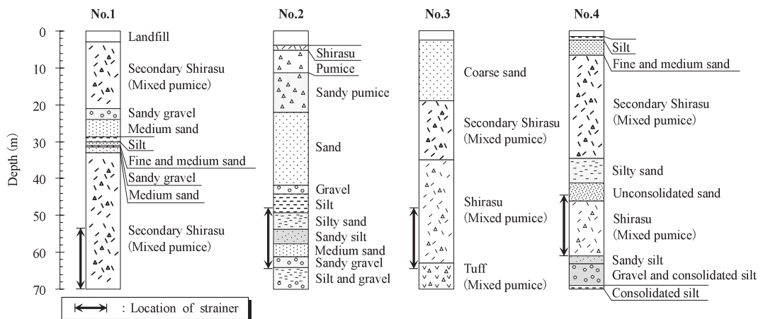
Fig. 2. Geological strata at four observation points in Kagoshima city
