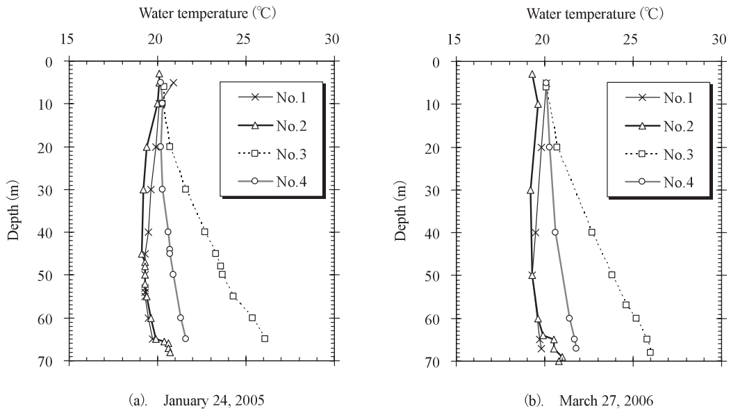
Fig. 9. Groundwater temperatures
