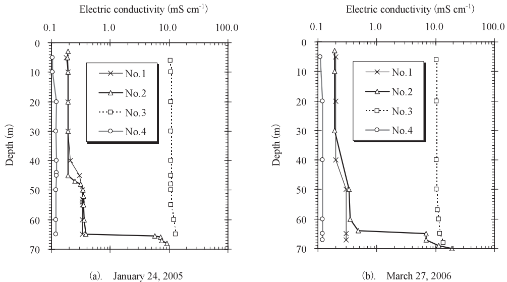
Fig. 8. Electric conductivities
