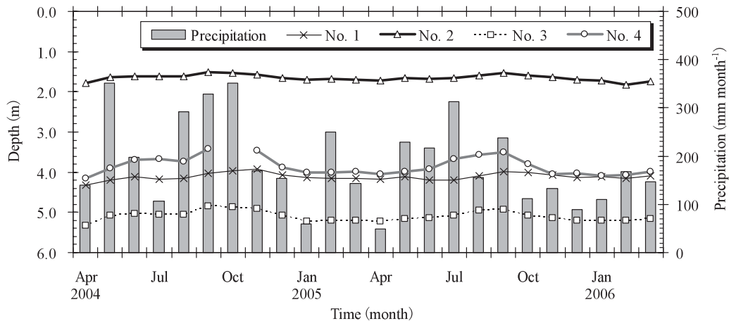
Fig. 5. Monthly changes in depths from the ground surface to the groundwater table and precipitation
