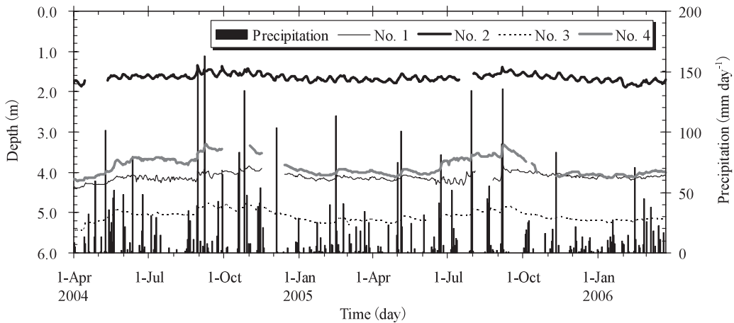
Fig. 4. Daily changes in depths from the ground surface to the groundwater table and precipitation
