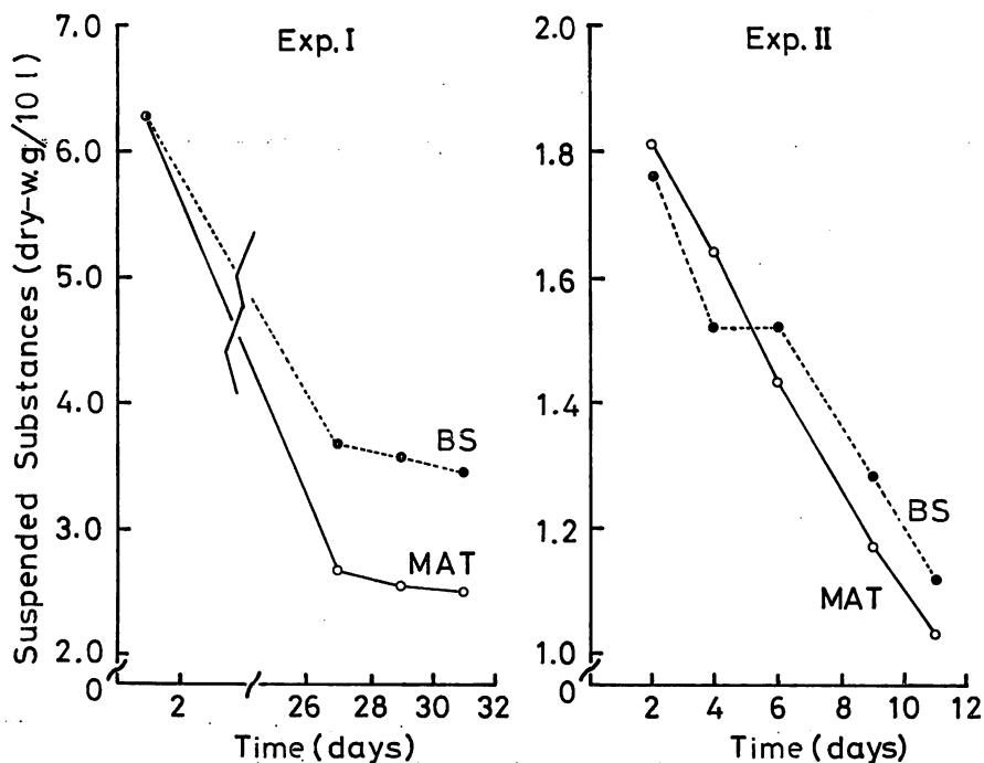
Fig. 3. Amount of suspended substances in 10 l of water in the tank aerated with bubbling stone and movable aerator tank.
