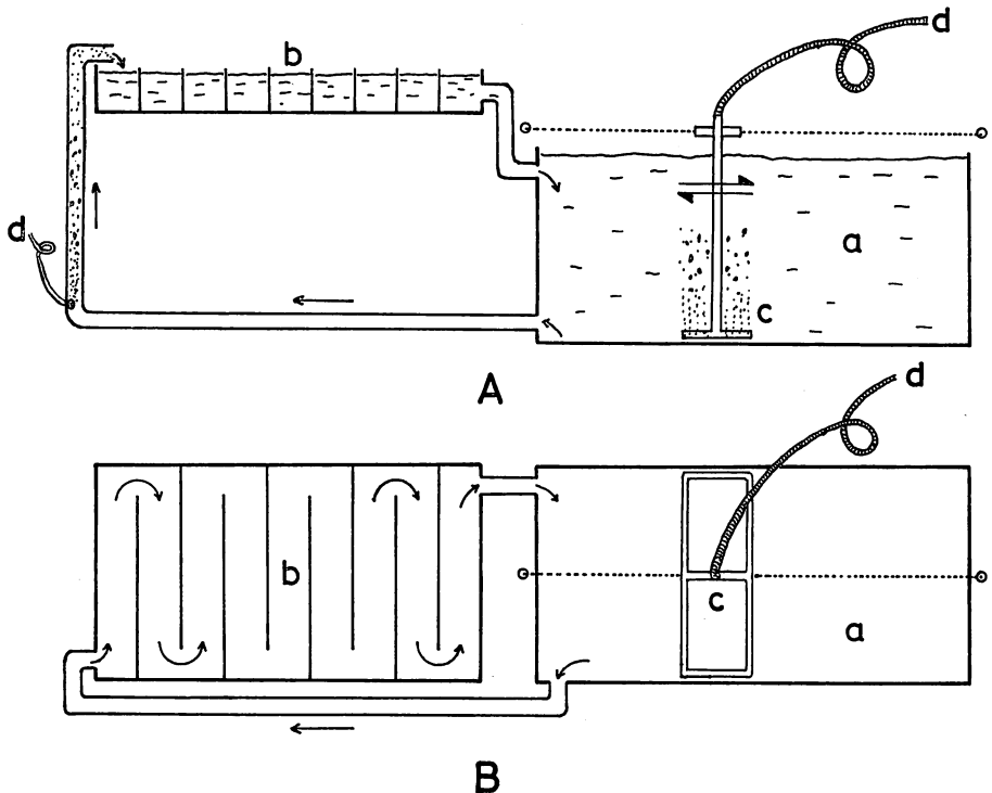
Fig. 1. Schematic diagram of experiment tank.
