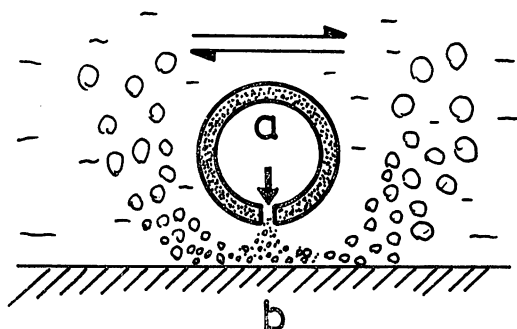
Fig. 2. Schematic diagram of movable aerator.
