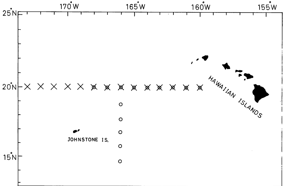
Fig. 1. Oceanographic stations of S. T. D observations in the southwestern waters of the Hawaiian Islands. circles, 1981; cross, 1982.
