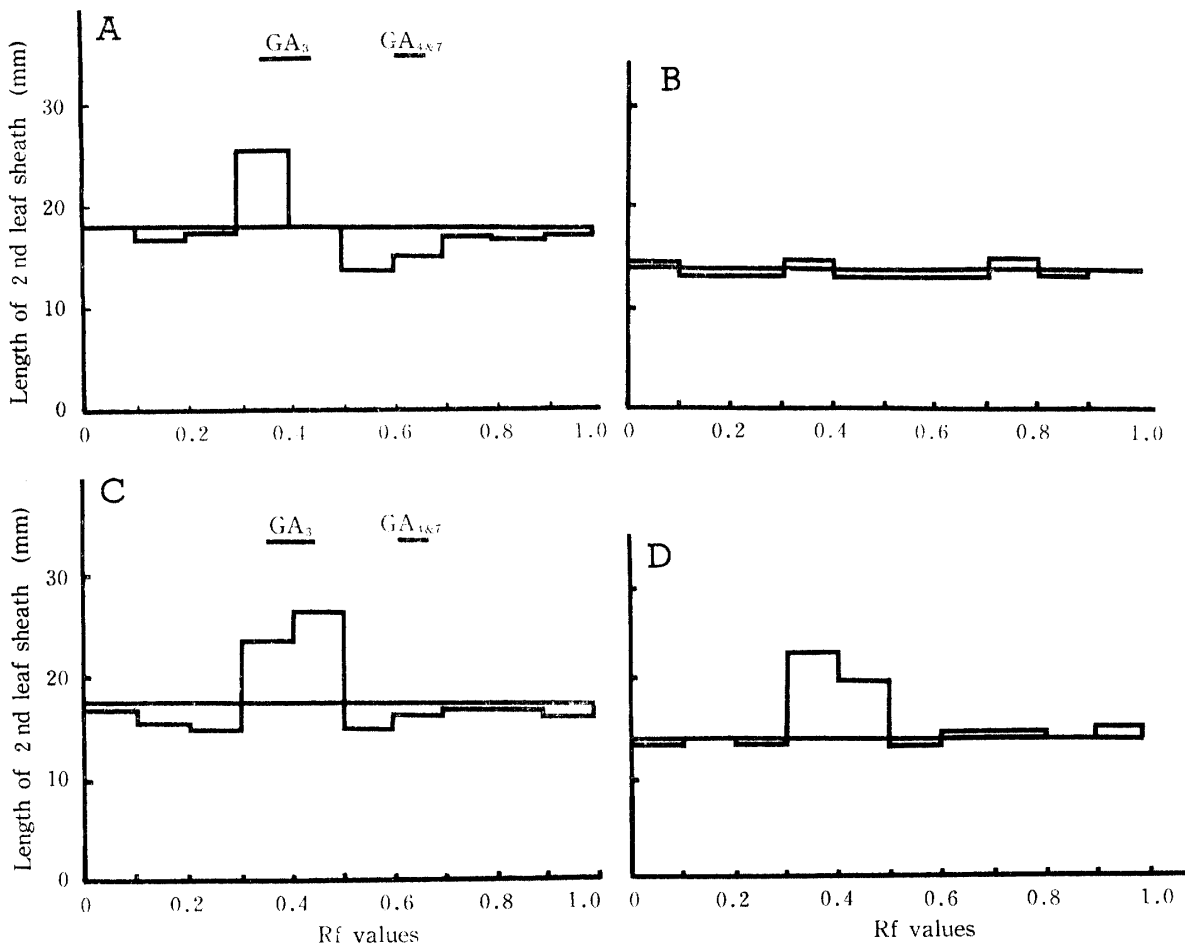
Fig. 5 A, B, C and D. GA-like activity of extract eluted by 40% ethyl acetate in n-hexane (A and B) and 45% ethyl acetate in n-hexane (C and D) in Fig. 4.
