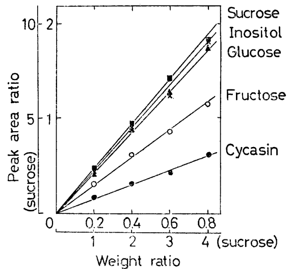
Fig. 1 Calibration curves for gas chromatography of cycasin and sugars.
