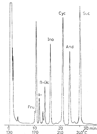
Fig. 2. Gas chromatogram of trimethylsilyl derivatives of the components found in cycad seeds.
