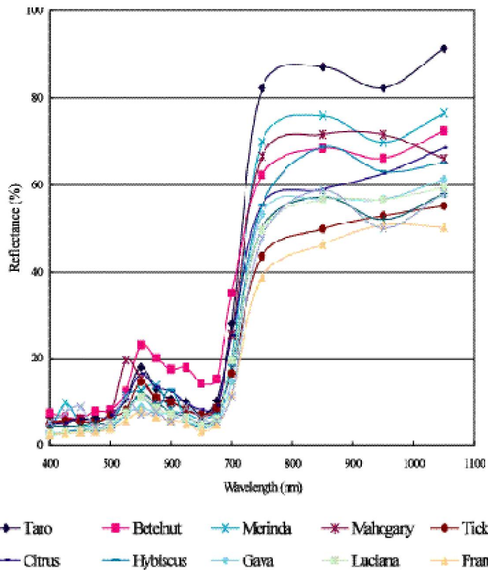
Fig. 7. Spectral reflectance on several crops.
