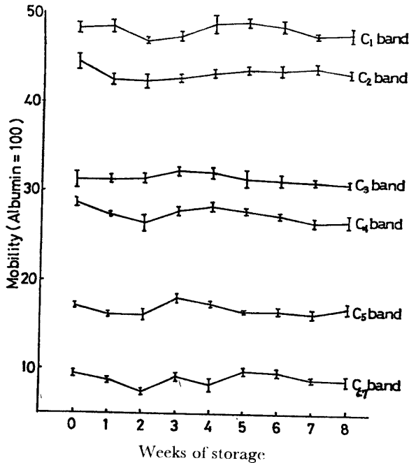
Fig. 1. Variation in the mobilities of horse serum cholinesterase isoenzymes after storage at -20^{\circ}\text{C} . The vertical bars represent each standard error.
