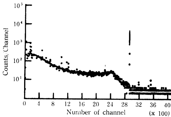
Fig. 1. Gamma spectrum for sample 3.
