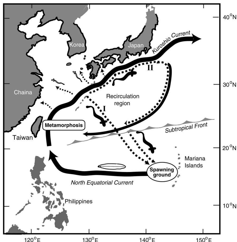
Fig. 7-1. Schematic drawing of the Japanese eel migration which is a round-trip journey between spawning and nursery grounds. Eel larvae or leptocephali passively drift with the oceanic currents. After metamorphosis, the glass eels orient towards the nursery grounds and acquire geomagnetic information in the process. After several years, the adult silver-phase eels leave continental coastal waters and head back to the North Pacific Ocean for spawning. Adult silver eels might return to the spawning grounds by first orienting eastward to the Kuroshio, then southeastward to the north equatorial Pacific. There are two ways to get across the Kuroshio: I, the direct southeastward course at depth, crossing under the Kuroshio Current perhaps below 200 m; II, the circular route, rejoining the surface Kuroshio Current northeastward, then southward in the gyre. At the Subtropical Front, which lies between 20°N and 30°N latitude, the eels may reorient south-southeastward grounds near the Marianas. to the spawning.
