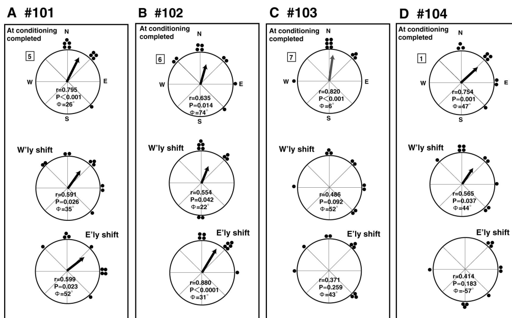
Fig. 5-7. Shelter choice orientation of four yellow eels at the completion of the reconditioning and changes in the orientation when the geomagnetic field was shifted westerly or easterly by the application of the artificial magnetic field at 31,063 nT. Figure in the square shows the number of conditioning runs at the conditioning was completed. These yellow eels had been conditioned and exposed twice to the artificial magnetic field at 192,473 nT.
