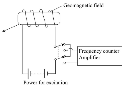
Fig. 1-2. Principle of proton magnetometer.
