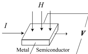
Fig. 1-1. Principle of magnetic field detection by Hall effect. I , electric current; V , induced voltage; H , magnetic field.
