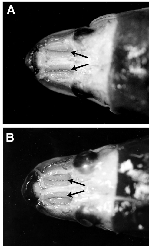
Fig.4-5. Photographs showing the olfactory rosette of Japanese eels: (A) control eel, (B) anosmic eel with white Vaseline injected into the nasal cavity.
