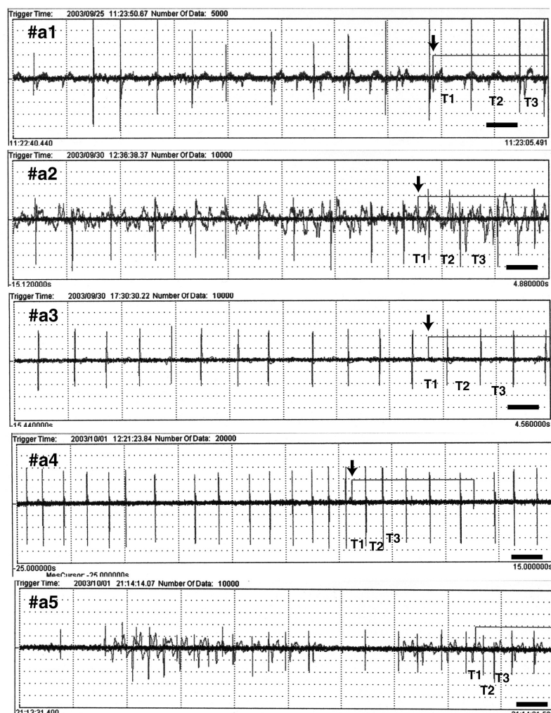
Fig. 4-4. Electrocardiograms showing the heart beats before and during conditioning tests in anosmic Japanese eels #a1 to #a5.
