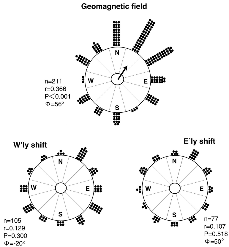
Fig. 6-4. Orientation of the glass eels in the testing tank under the geomagnetic field and artificial magnetic field applied westerly and easterly. n, number of glass eels excluding specimens remained in the release device.
