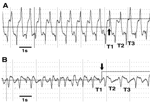
Fig. 3-6. Typical electrocardiograms showing the conditioned response (slowing down of the heart beat) of glass eels during tests following a set of conditioning runs. Horizontal bars mark the magnetic field stimulus. T1, T2, and T3 are the heart beats during the conditioning tests at (A) 192,473 nT and at (B) 12,663 nT.
