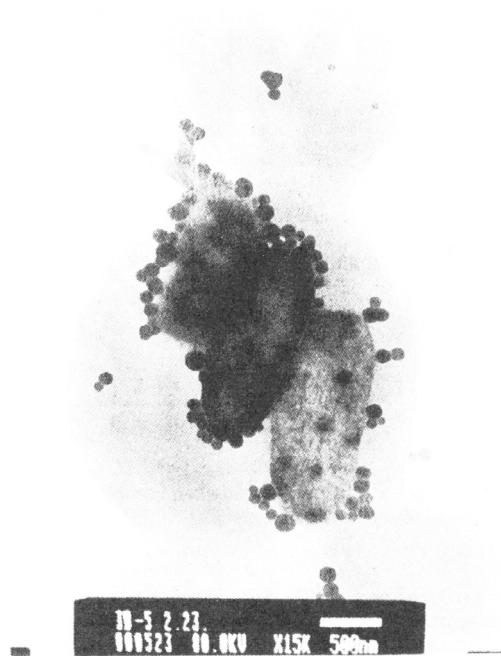
Fig. 2-1. Transmission electronmicrograph showing a candidate for biomagnetic sense organ extracted from the forehead of sockeye salmon. Three elliptical cells are encircled by numerous small magnetic particles linking as chains in a semitransparent tube-like tissue. The minor and major axes of the cells are about 0.65-0.75 \mu m and 1.3-1.8 \mu m, respectively. Scale bar, 0.5 \mu m. (from Sakaki et al. , 1990).
