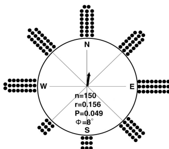
Fig. 5-5. Shelter choice orientation for combined fifteen yellow eels in the testing tank under the geomagnetic field. Symbols, same as in Fig. 5-4.
