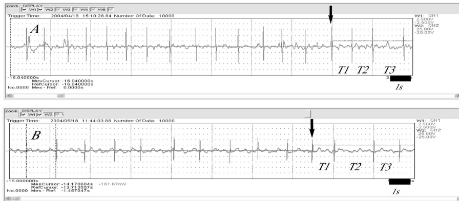
Fig. 4-3. Typical electrocardiograms showing the conditioned response (slowing down of the heart beat) of yellow eels during tests following a set of conditioning runs. Horizontal bars mark the magnetic field stimulus. T1, T2, and T3 are the heart beats during the conditioning tests at (A) 192,473 nT and at (B) 2,533 nT.
