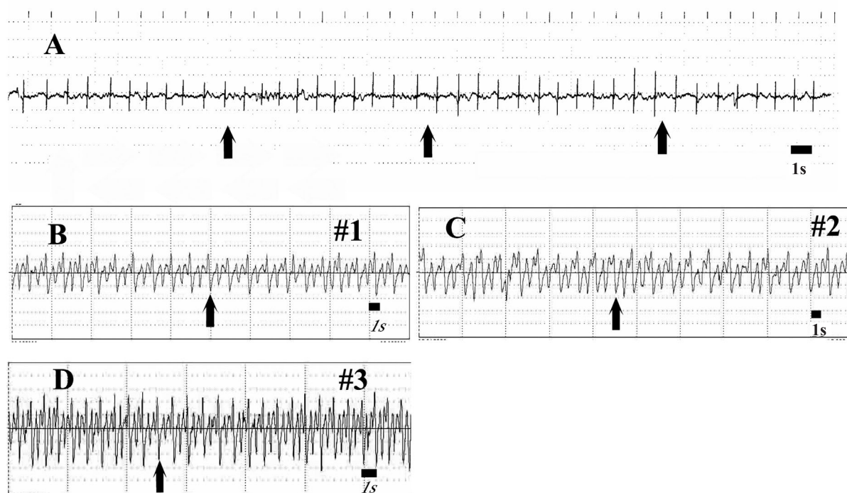
Fig. 3-1. Electrocardiograms recorded from unconditioned yellow eel (A) and glass eel (B-D). Arrow, onset of artificial magnetic field given for 2s; horizontal bar, 1s. Note that there was no cardiac change in response to the magnetic field stimulation.
