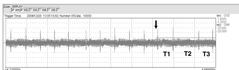
Fig. 5-8. Electrocardiogram showing the conditioned response of yellow eel #3 during a test following 3 sets of conditioning runs. This specimen was not able to condition to choose a north shelter in the test tank.
