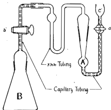
A: reaction vessel B: absorption flask a & b: 2 way stop-cocks
