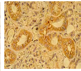
図-6 P-gp
