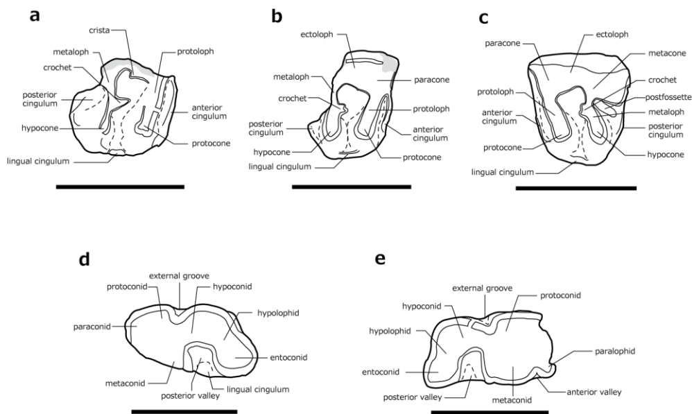
Figure 9. Schematic drawing of the cheek teeth of Brachytherium cf. minor .
