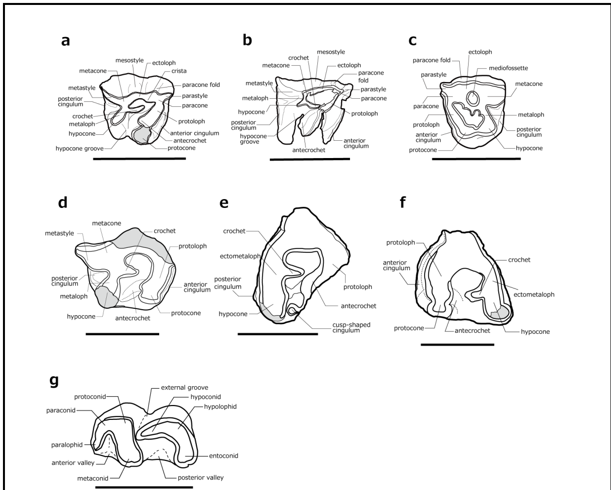
Figure 4. Schematic drawing of the teeth of Chilotheridium pattersoni .
