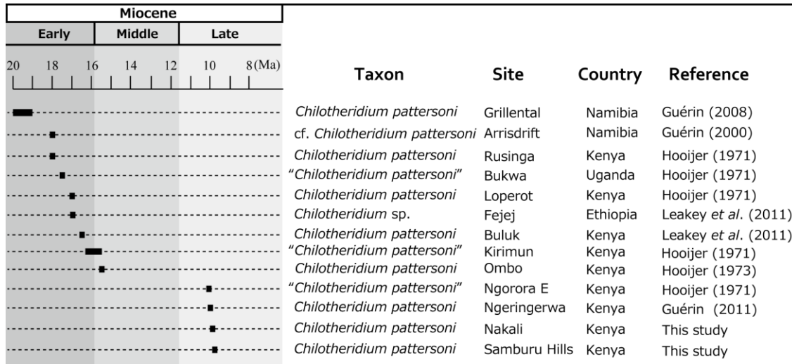
Figure 5. Temporal range of Chilotheridium pattersoni in sub-Saharan Africa.
