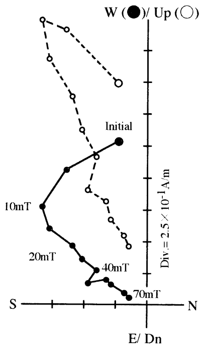
Figure 6. Typical AF demagnetization plots on vector component diagrams for the Togo Andesites.
