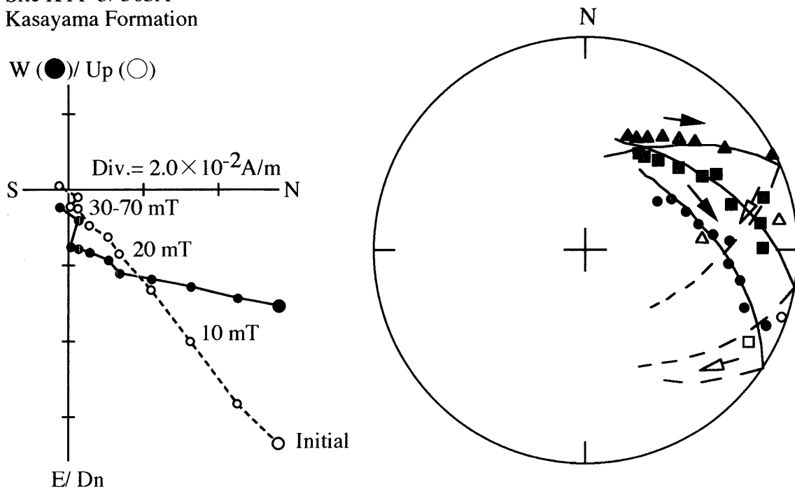
Figure 5. Typical vector component diagram (left) and equal-area projection (right) for the Kasayama Formation.
