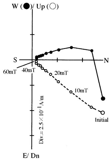
Figure 6. Typical AF demagnetization plots on vector component diagrams for the Togo Andesites.
