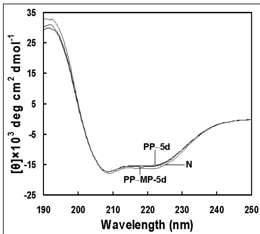
Figure 2—CD spectra of BSAs. For definitions of N, PP, and PP–MP, see Figure 1.
