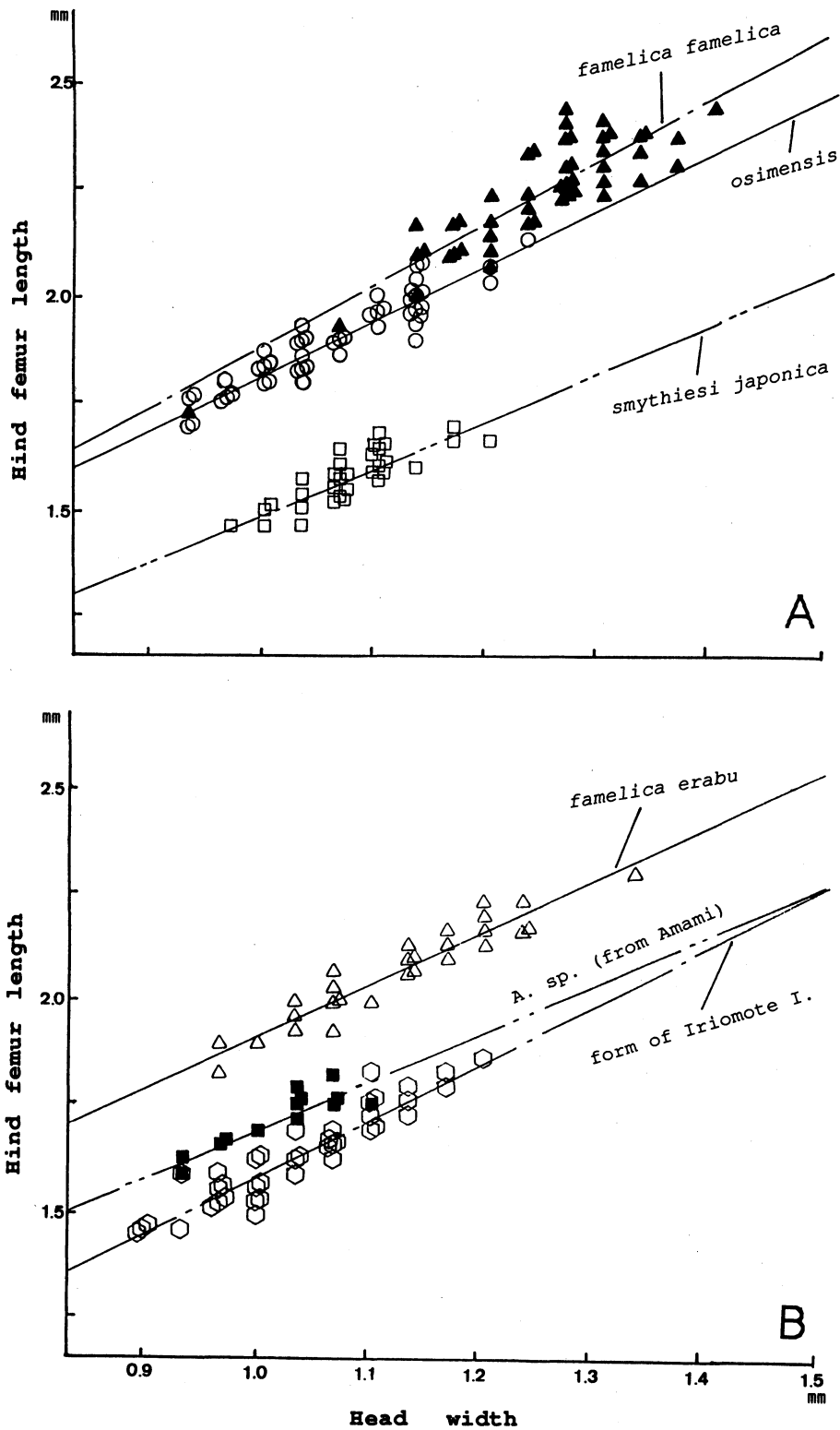
Fig. 4. Hind femur length against head width (worker) in six forms of Aphaenogaster from Japan.
