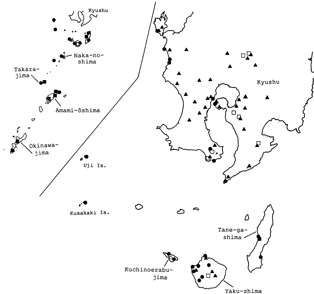
Fig. 7. Distribution of Aphaenogaster forms in Kagoshima-ken-hondo (mainland) and the N. and C. Ryukyus. Symbols as in Fig. 8. Black squares: Amami-type.
