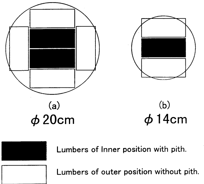
Fig. 1. Sawing Patterns. Legend : φ : Diameter at top end.
