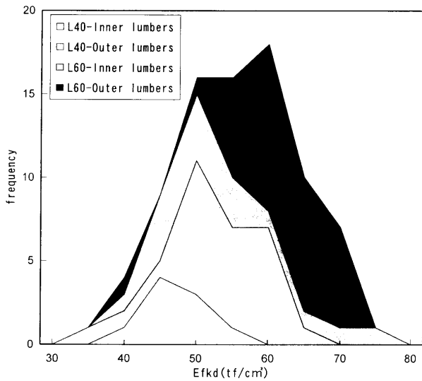
Fig. 5. Distribution frequency of selected EfkD by using together of grading for Efl and sawing position.
