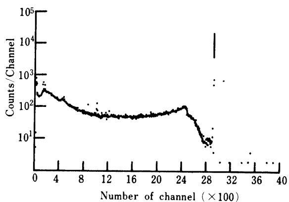
Fig. 1 Gamma spectrum of potassium chloride.
