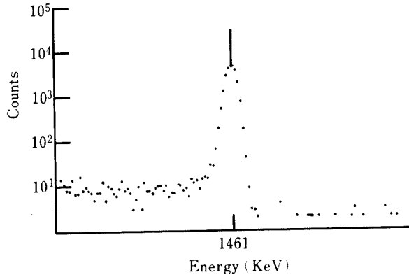
Fig. 2 Peak shape of ^{40}\text{K} gamma ray.
