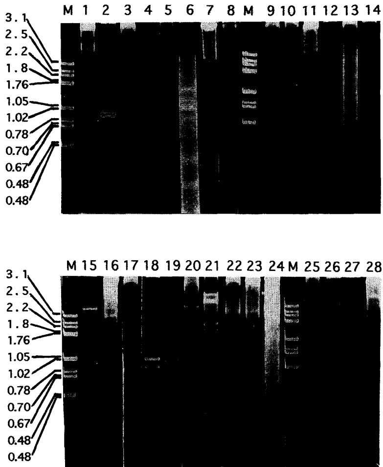
Fig. 1 Electrophoresis of dsRNA preparations from various sources.
