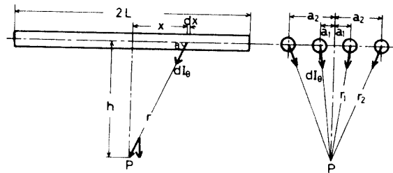
Fig. 2. Arrangement of ultraviolet lamps in the irradiation-apparatus.
