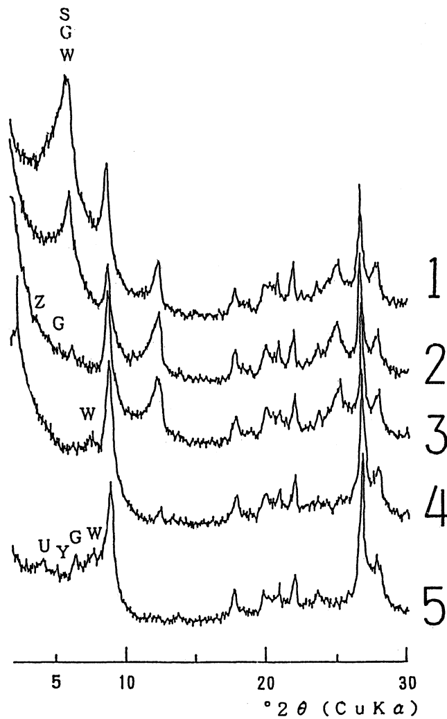
Fig. 9 XRD patterns of specimen D-1 after heating at various temperatures for 1 hr.
